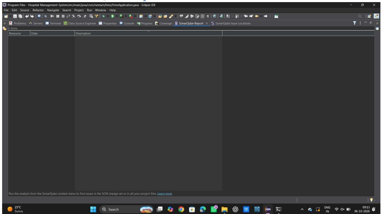
Figure 2.3: SonarQube Report
